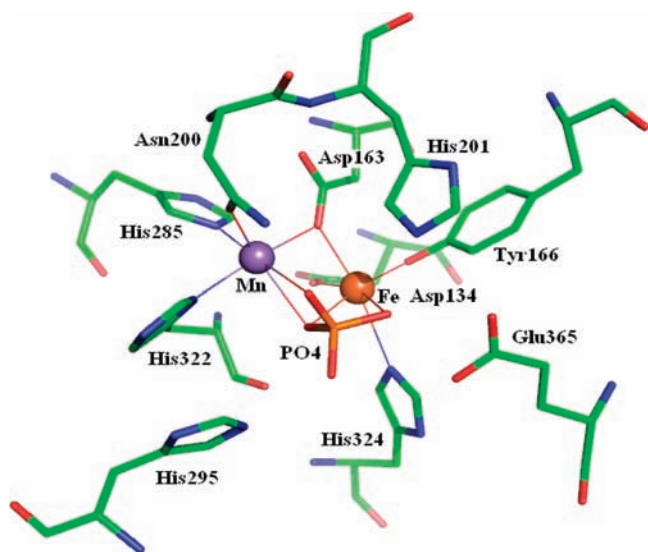
Figure 1. Schematic illustration of the active site of FeMn-spPAP. 13e His201, His295, and Glu365 assist in substrate binding and orientation. The substrate analogue (PO 4 ) is shown in a possible transition state whereby the bridging oxygen acts as a nucleophile.
